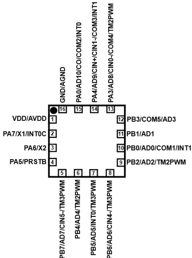
PMS120-1J16A: QFN3*3-16pin (0.5pitch)
